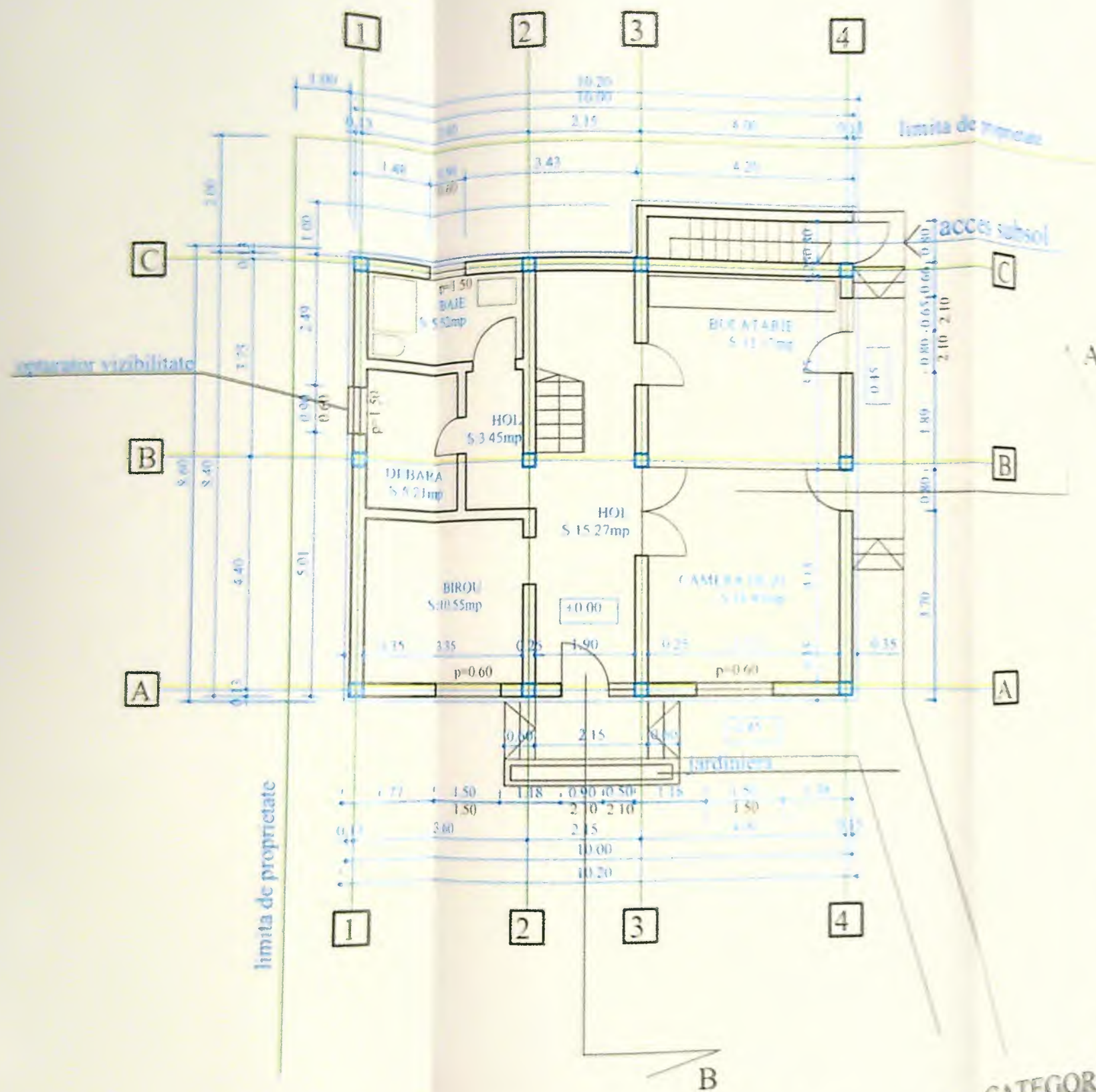
PLAN PARTER
